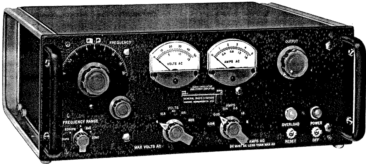
Figure 1-1. Type 1308-A Audio Oscillator and Power Amplifier.
