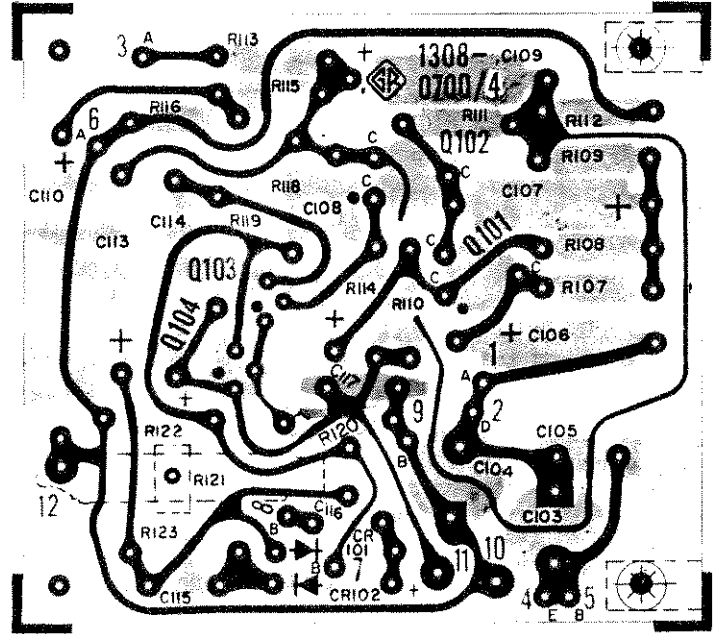
Figure 5-4. Oscillator etched-circuit board.
