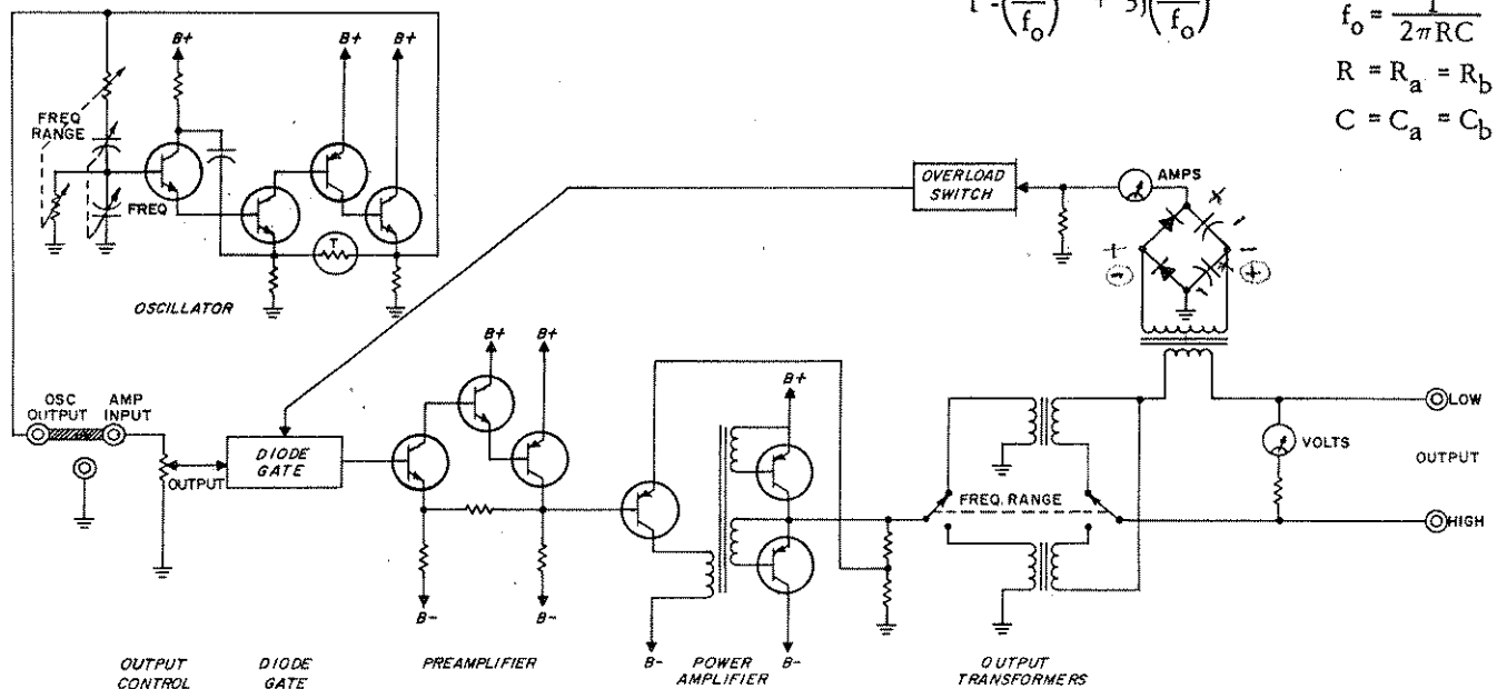
Figure 4-1. Elementary circuit diagram for Type 1308-A Audio Oscillator and Power Amplifier.
