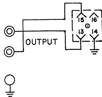
Figure 2-2. Output connections.
